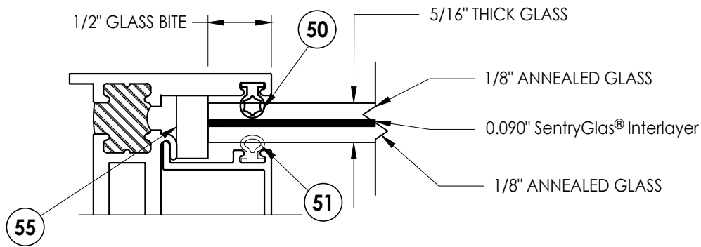
G4 GLAZING DETAIL
