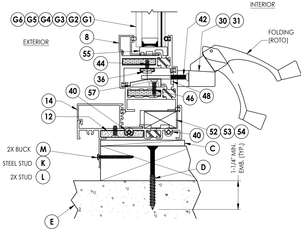
2 4 VERTICAL CROSS SECTION 2X Buck Construction Shown w/ nailing fin option
