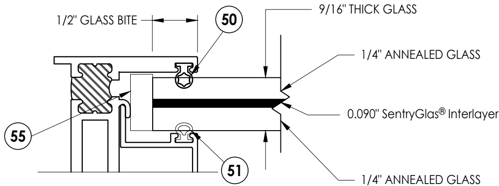
G6 GLAZING DETAIL
