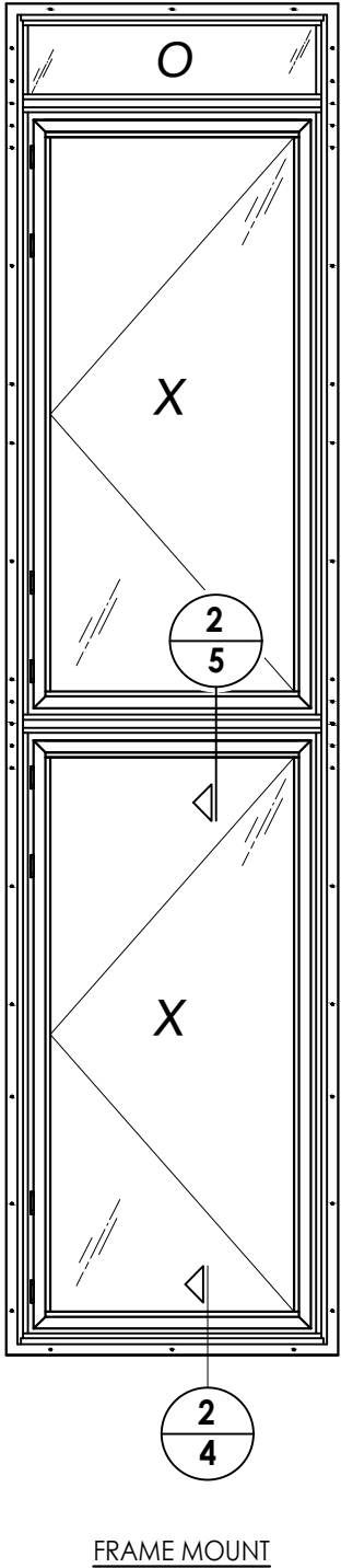
FRAME MOUNT
