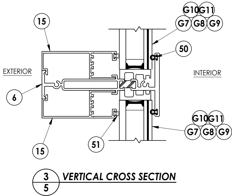
1 5 VERTICAL CROSS SECTION
